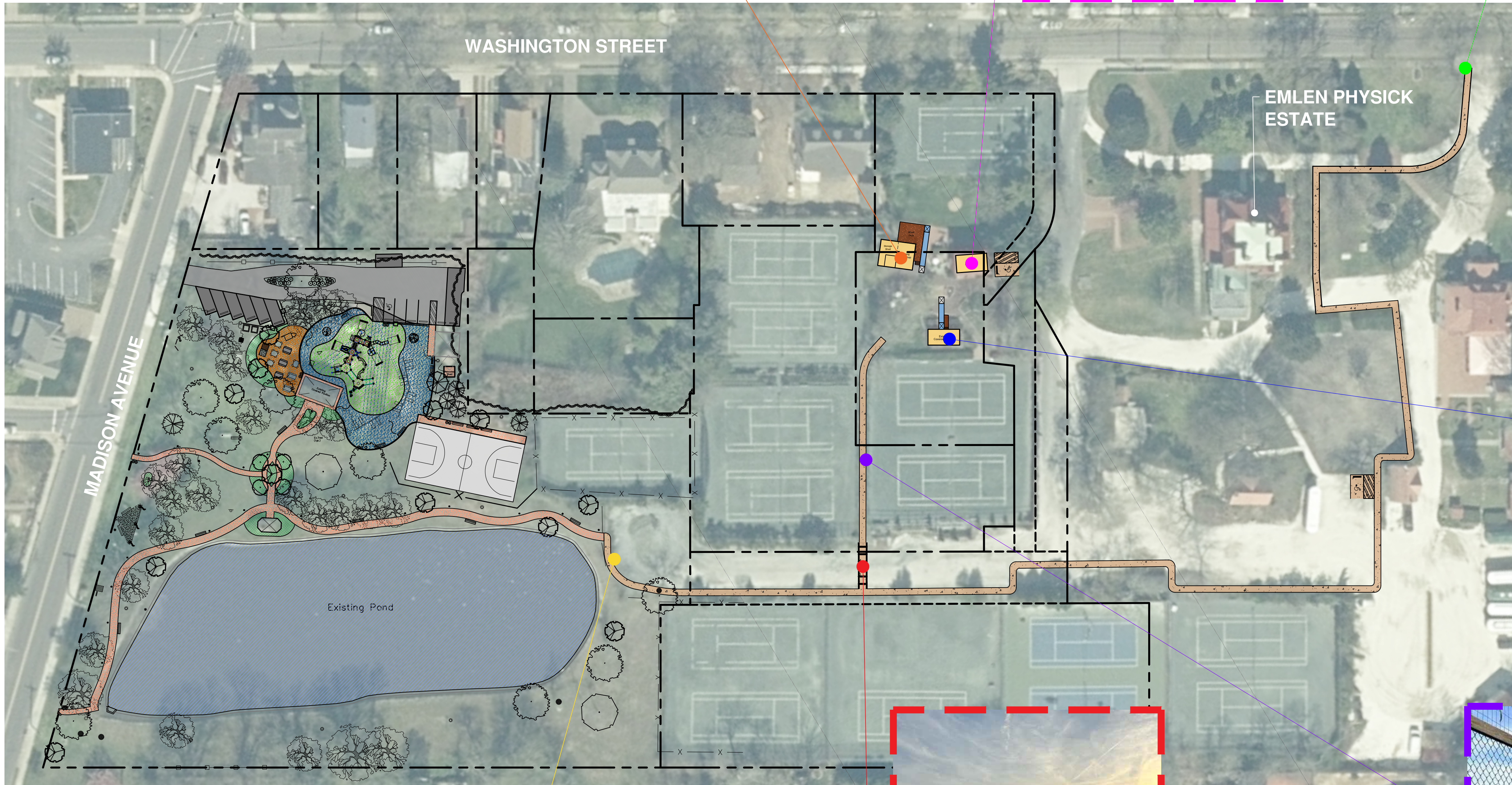
CONSTRUCT ADA ACCESSIBLE PATHWAY TO ADA CROSSWALK RAMP ON WASHINGTON STREET
